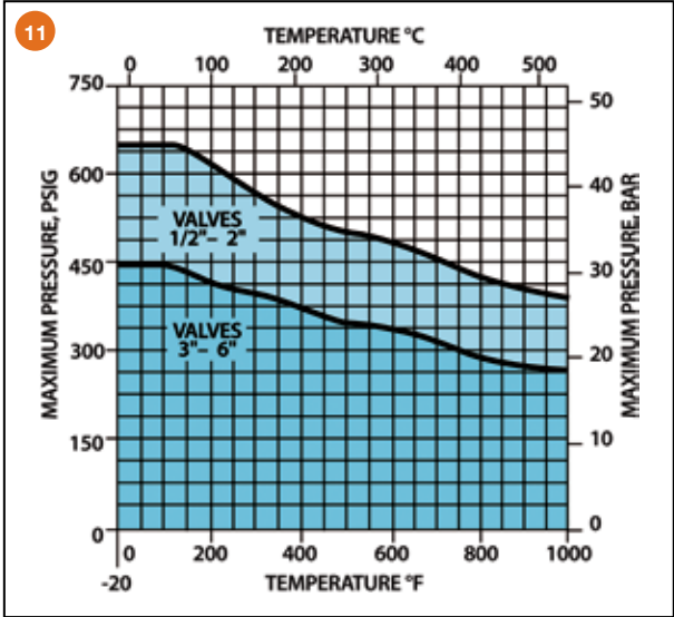
Figure 9. Bellows Seal Rating Chart
